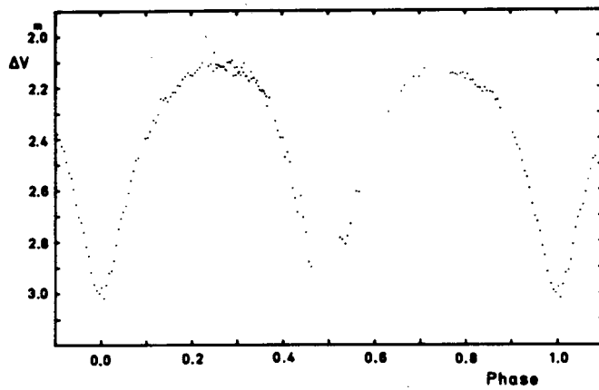
Fig. 2 V observations of BF Pav
