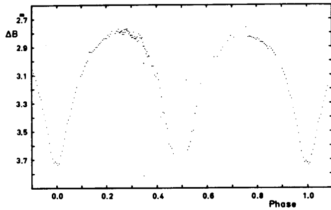
Fig. 1 B observations of BF Pav
