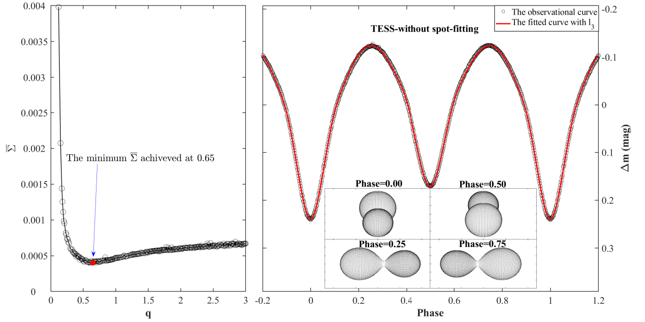
Figure 5. The diagram of without-spot fitting obtained using the W-D program. Left panel: the relation between q and \bar{\Sigma} determined by model 3 for TESS. Right panel: the observation light curves (the black circles), the theoretical fitting light curves with the third light l_3 (the red solid line), and the theoretical geometrical structure for TESS.
