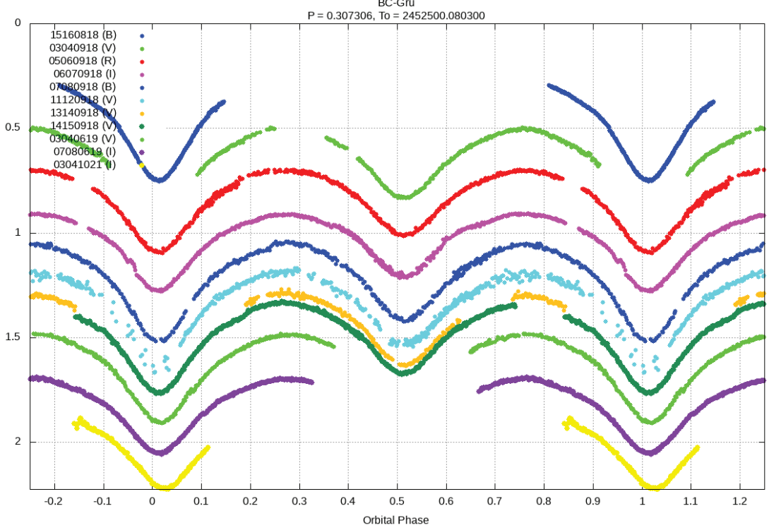
Figure 1. The phased eclipsing light curves observed at CASLEO, where different color lines represent different observational dates.
