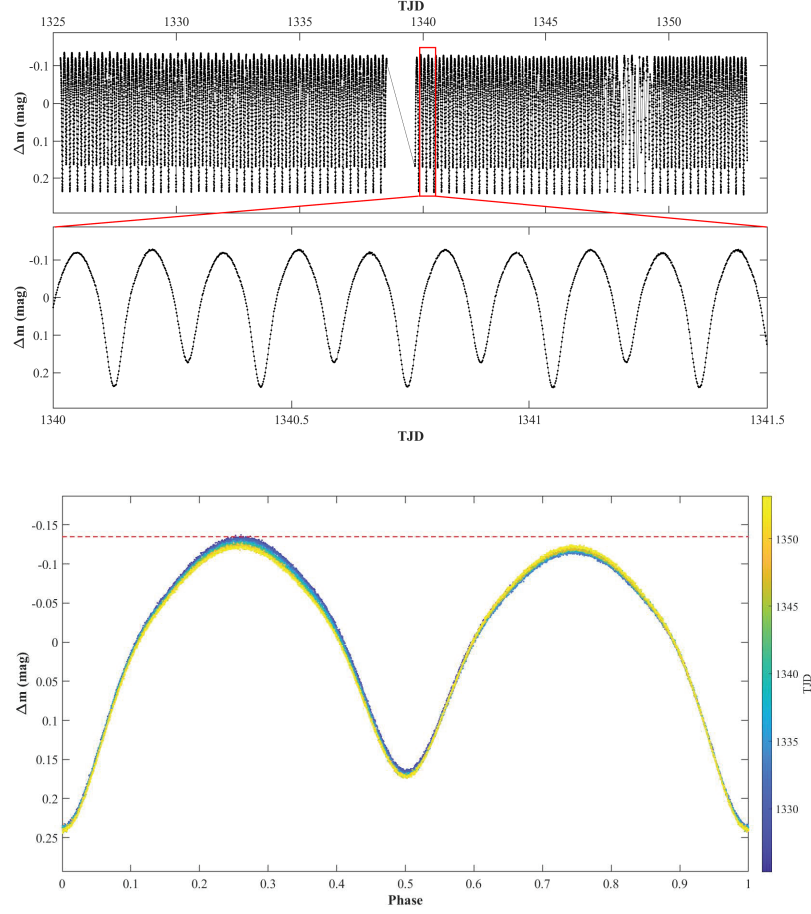
Figure 2. The TESS LCs of BC Gru with an interval of 2 minute cadence (TJD = BJD-2457000.0), where the details of light curve for five cycles are also displayed in middle. Bottom panel: the phased TESS LCs, where the color variation from dark blue to yellow represents changes over the time.
