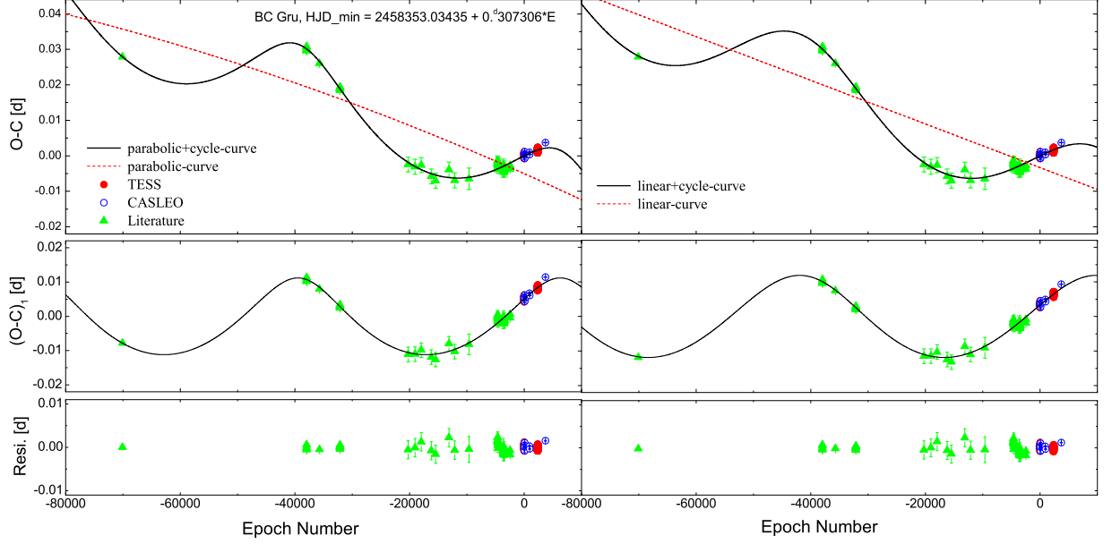
Figure 3. The (O - C) diagrams of BC Gru fitted with an eccentric orbit: left panels for the pattern of parabolic plus cyclical fit, while right panels for that of linear plus cyclical fit. The data sources and colored lines are noted in the upper panels, the cyclical variations alone are shown in the middle panels, and the residuals from the whole effect are displayed in the bottom panels.
