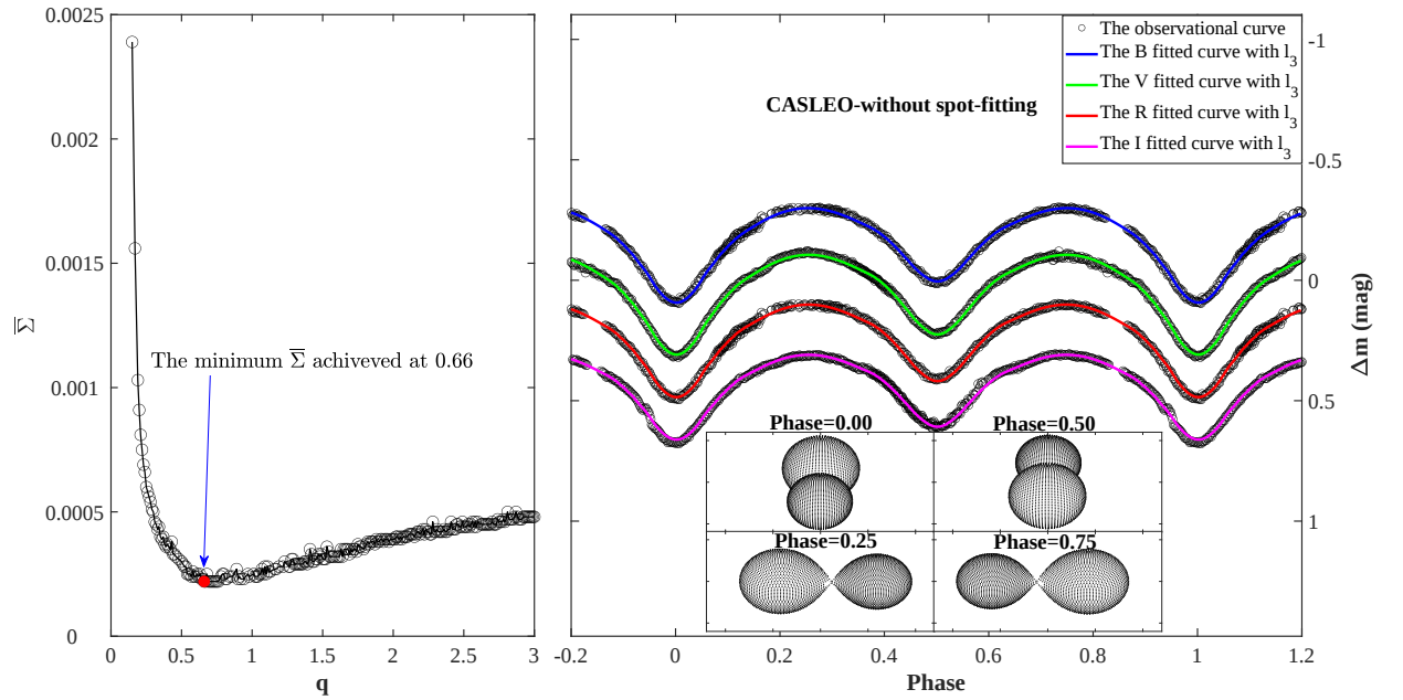
Figure 6. Same as the Fig. 5, but for CASLEO LCs fitting.
