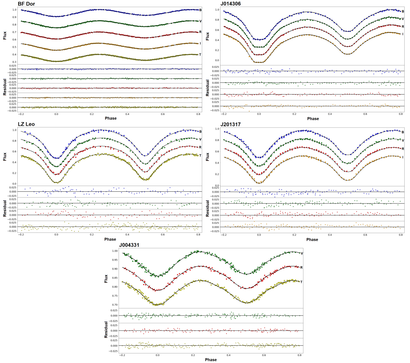
Figure 4. The colored dots represent the observed light curves of the systems in different filters, and the synthetic light curves, generated using the light curve solutions, are also shown. Residuals are shown at the bottom of each panel.
