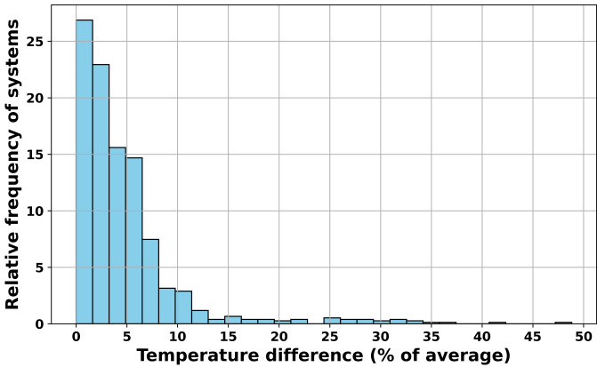
Figure 7. Histogram showing the relative frequency distribution of temperature difference percentages among contact binary systems. The x-axis represents the temperature difference as a percentage of the average component temperature, while the y-axis shows the fraction of systems in each bin.
