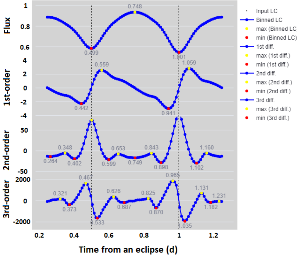
Figure 7. A photometric light curve of V0801 And, and first to third derivatives (top to bottom panels, respectively) as an example of a process for systems. The units of the panels on the vertical axis from top to bottom are \text{W m}^{-2} , 10 \text{ W m}^{-2} \text{ day}^{-1} , 10^2 \text{ W m}^{-2} \text{ day}^{-2} , and 10^4 \text{ W m}^{-2} \text{ day}^{-3} , respectively.
