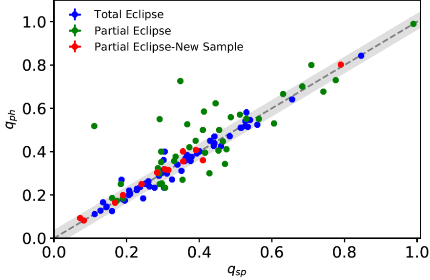
Figure 6. Comparing mass ratio results utilizing spectroscopic ( q_{sp} ) and photometric ( q_{ph} ) data for available samples.
