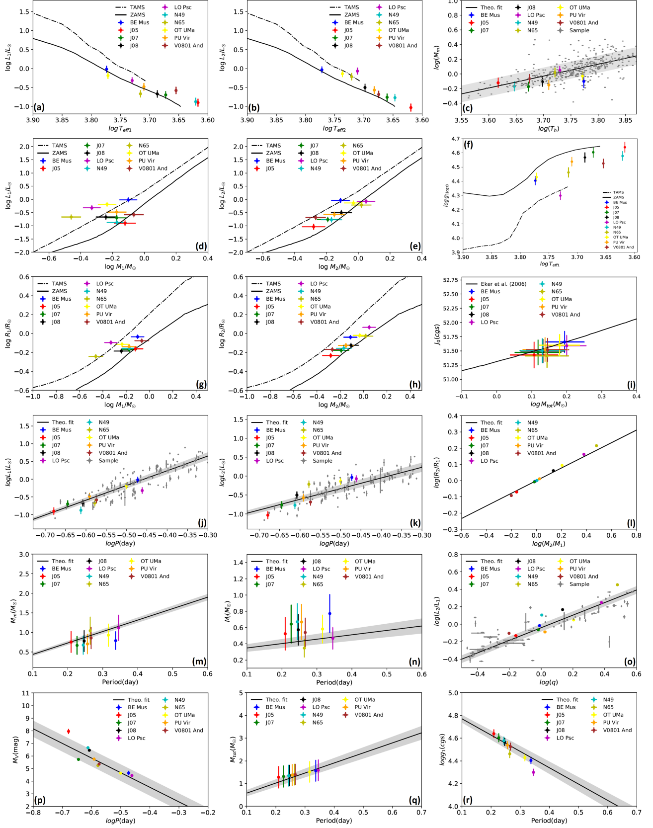
Figure 8. The position of the target systems in different diagrams of the parameter relationships.
