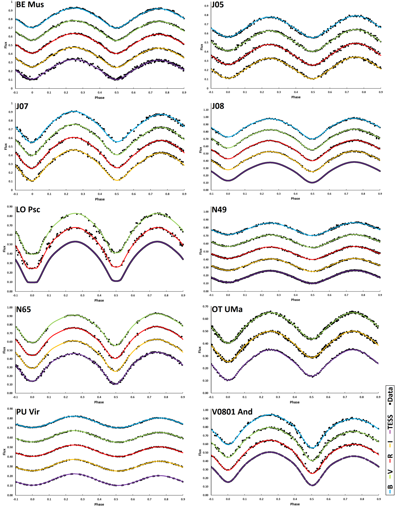
Figure 4. The black dots show the observed light curves of the systems, and the synthetic light curves were generated using the light curve solutions. From top to bottom, the filters are B , V , R , I , and TESS, as shown by the colors.
