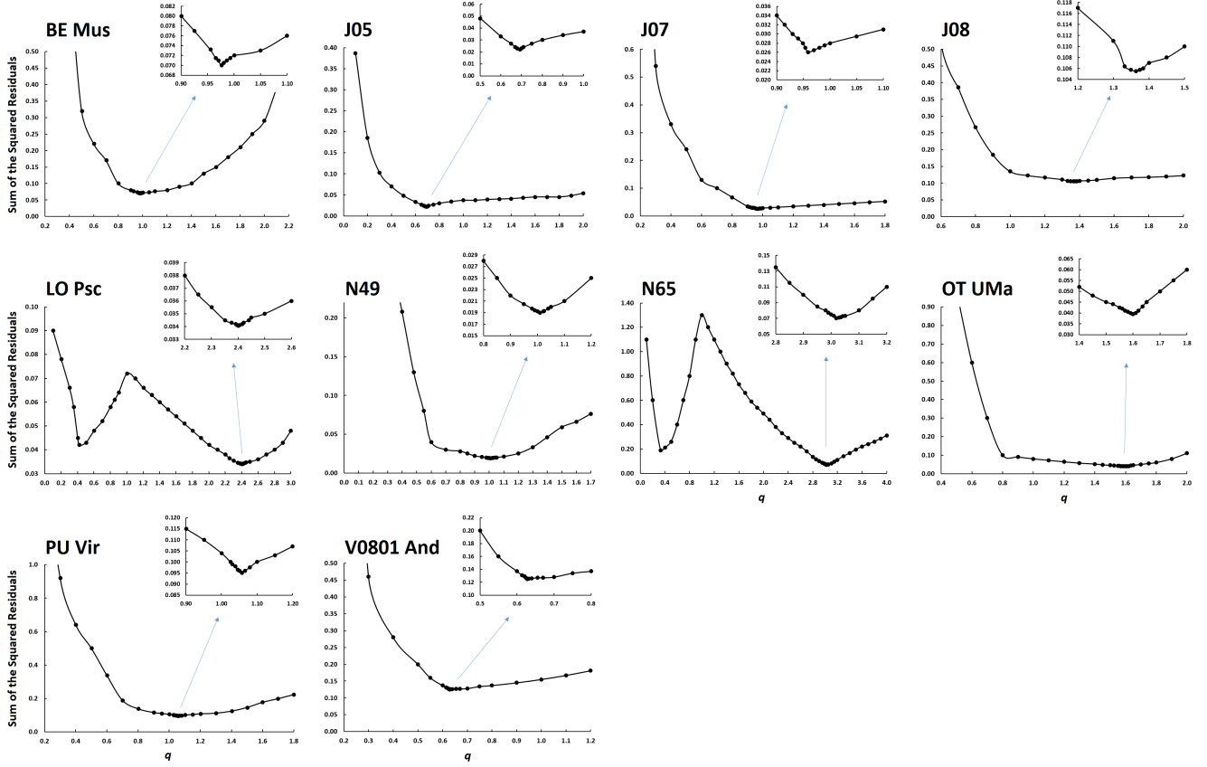
Figure 2. Sum of the squared residuals as a function of the mass ratio. The zoomed part is shown with an arrow.
